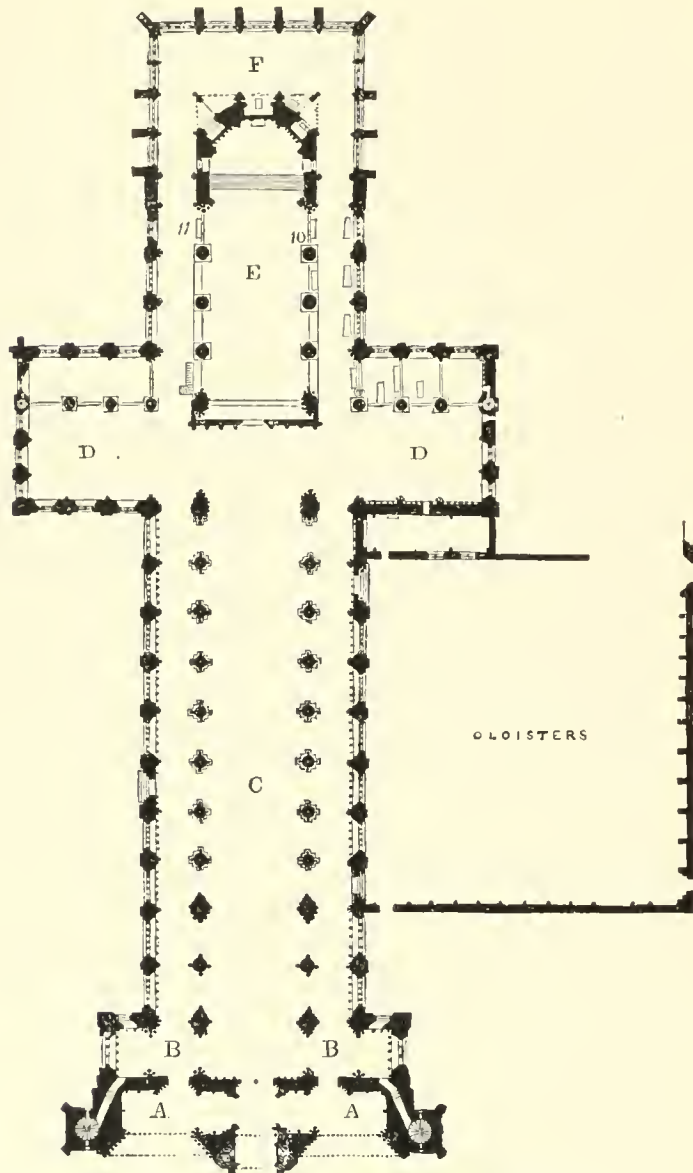
PLAN OF PETERBOROUGH CATHEDRAL. 1
